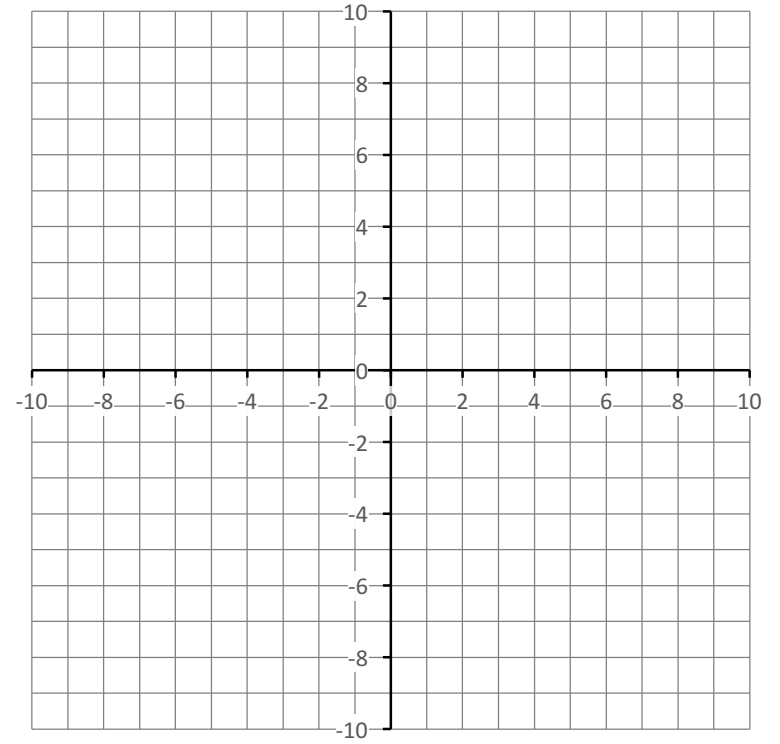
Four quadrant grid (-10 to 10)
